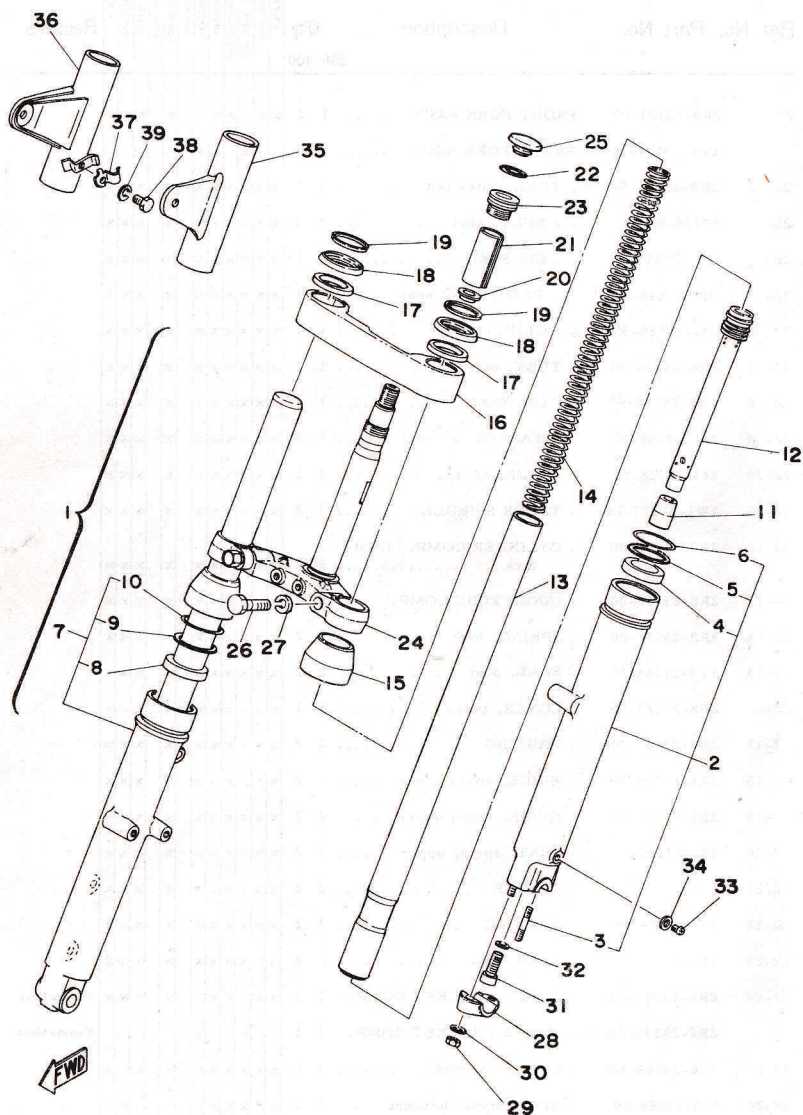
Fig. 22 FRONT FORK
