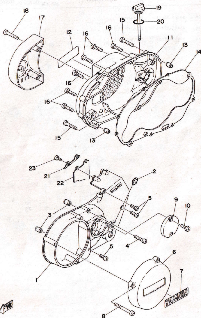
Fig. 3 CRANKCASE COVER
