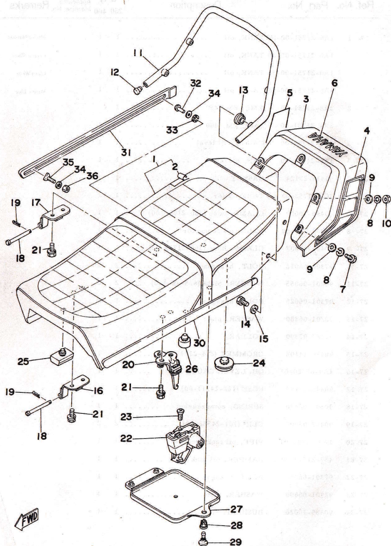
Fig. 28 SEAT
