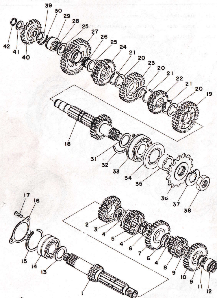
Fig. 6 TRANSMISSION
