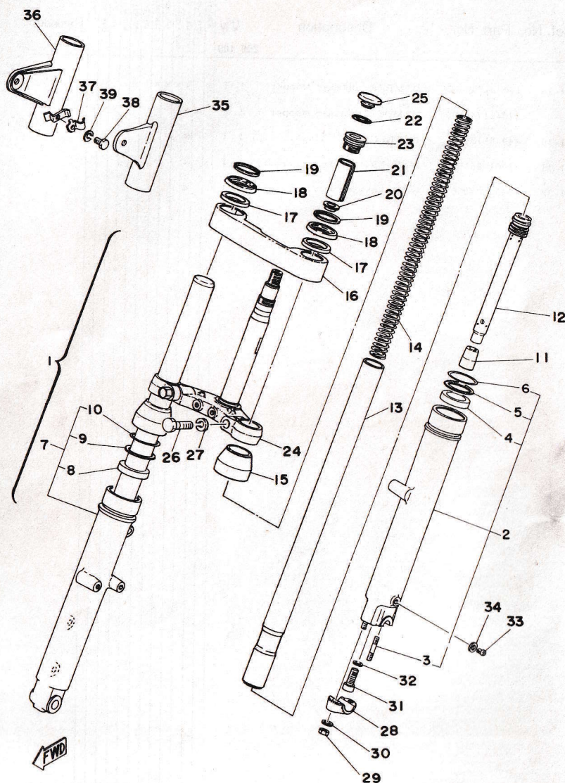
Fig. 22 FRONT FORK
