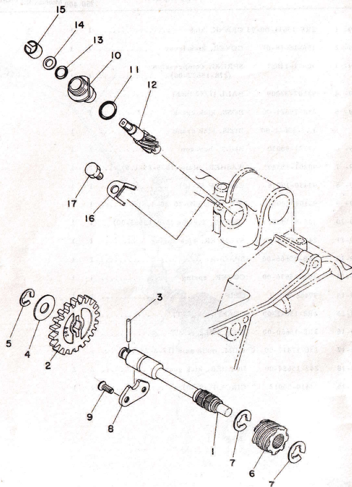
Fig. 10 TACHOMETER GEAR
