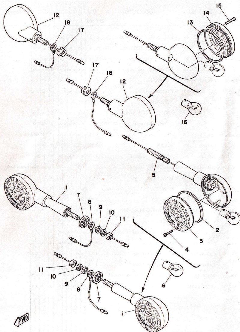
Fig. 40 FLASHER LAMP 1
