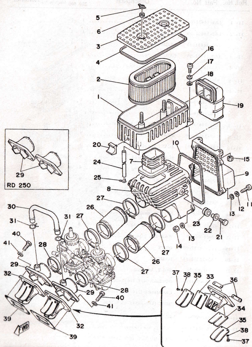
Fig. 11 INTAKE
