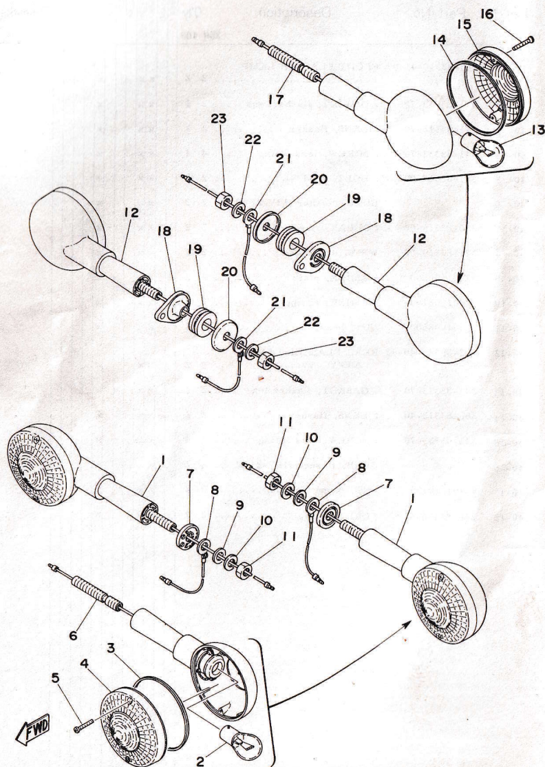
Fig. 41 FLASHER LAMP 2
