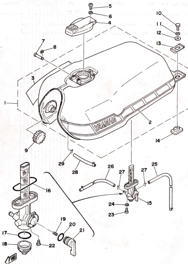
Fig. 26 FUEL TANK
