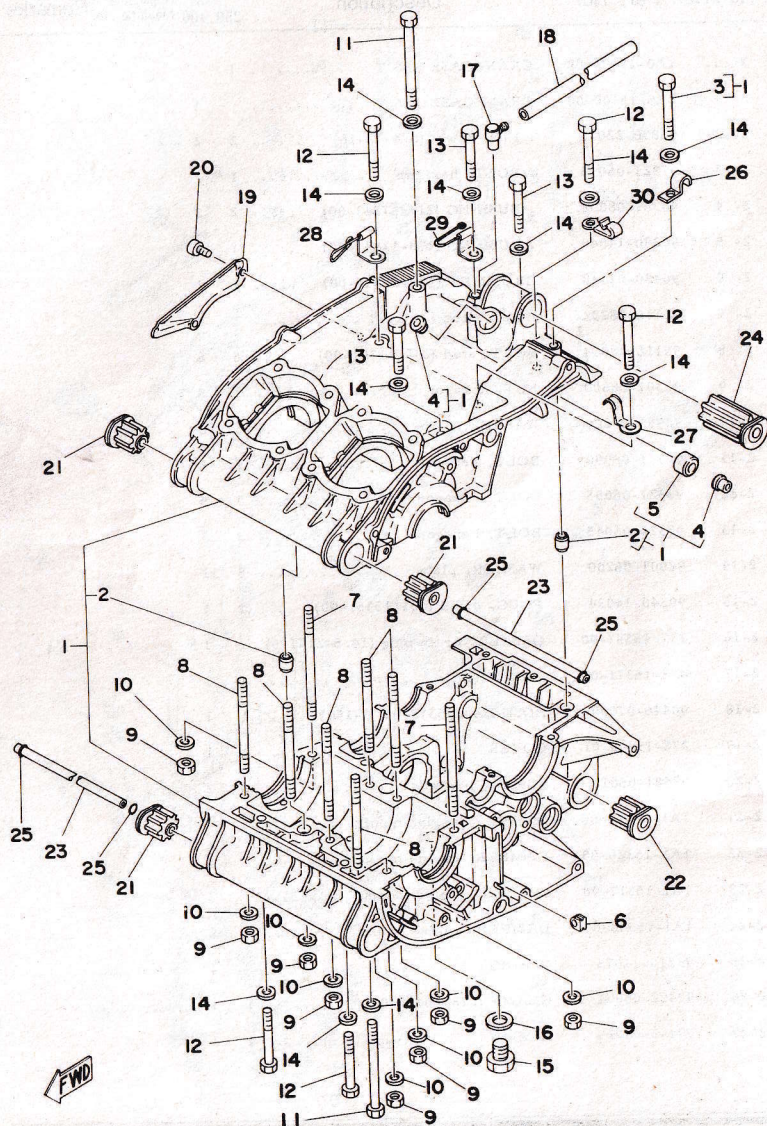
Fig. 2 CRANKCASE
