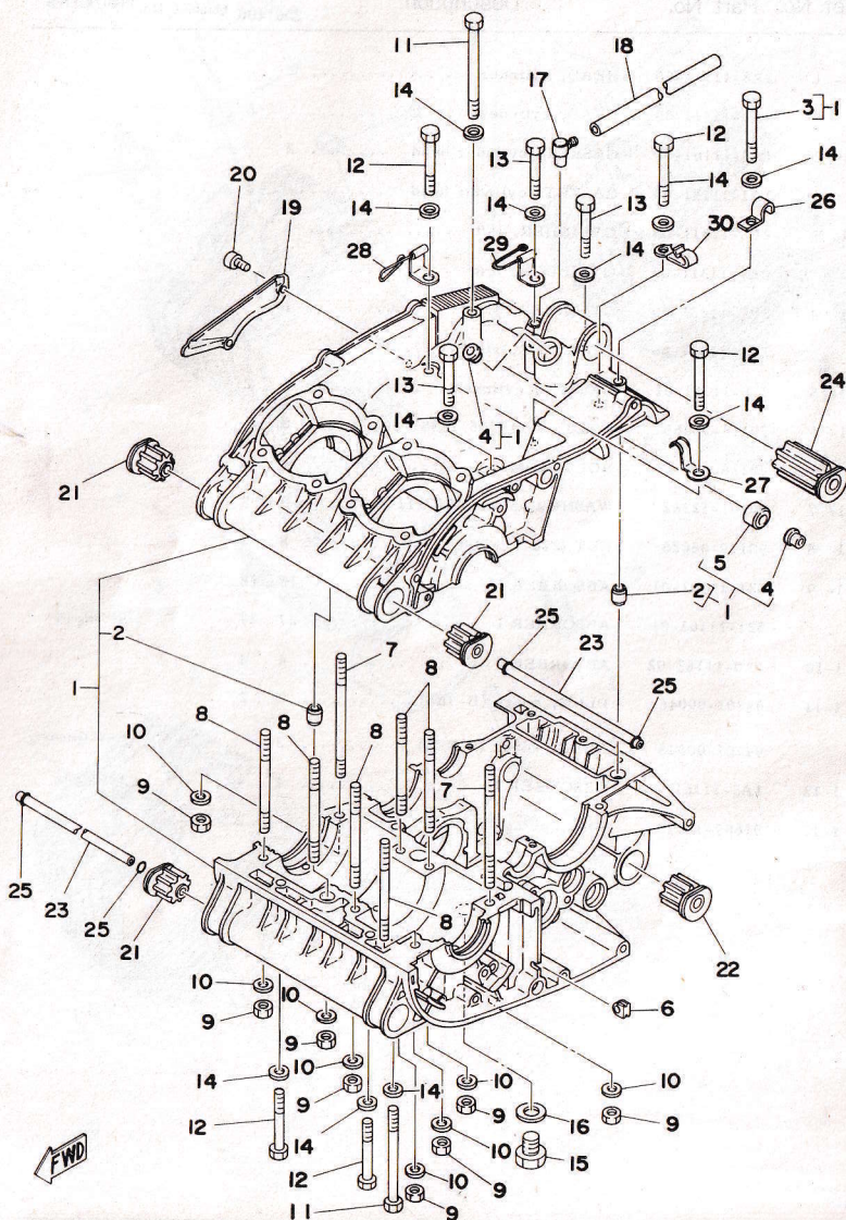
Fig. 2 CRANKCASE
