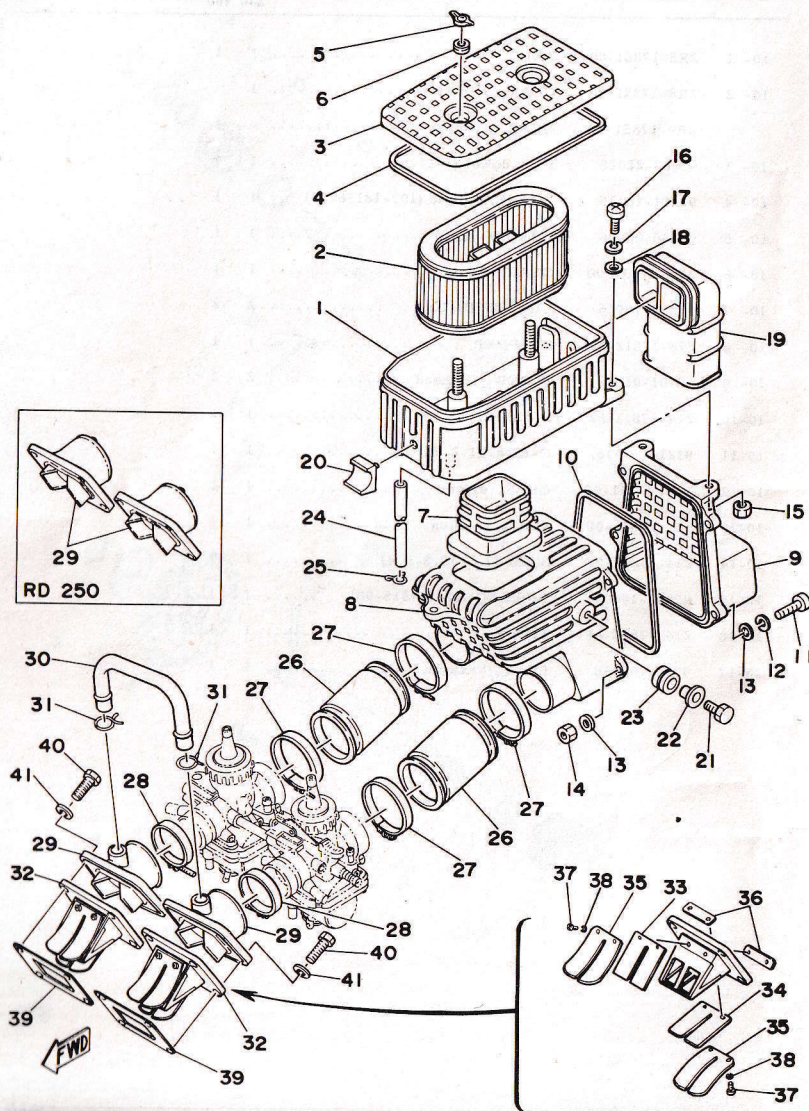
Fig. 11 INTAKE
