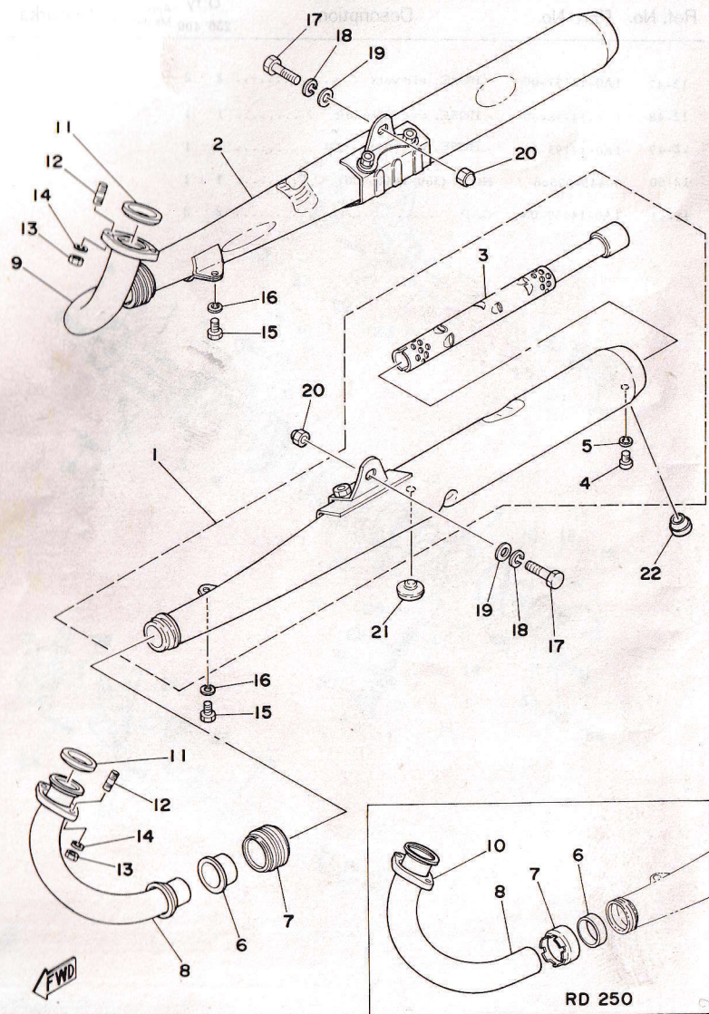
Fig. 13 EXHAUST
