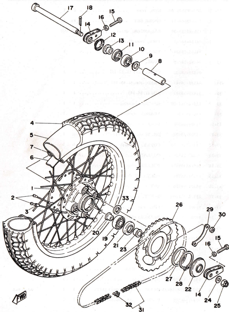
Fig. 33 REAR WHEEL (SPOKE WHEEL TYPE (ALTERNATE PARTS ENGLAND ONLY))
