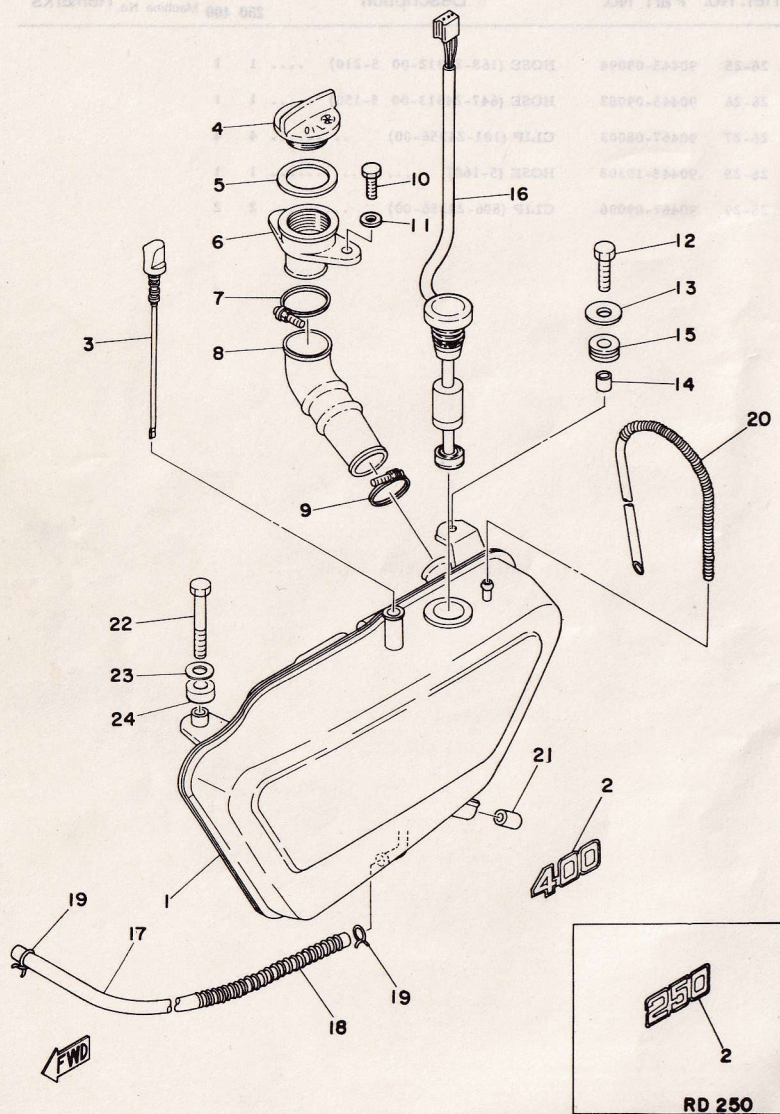
Fig. 27 OIL TANK
