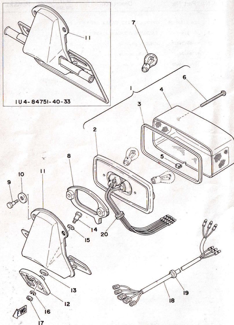
Fig. 39 TAIL LAMP
