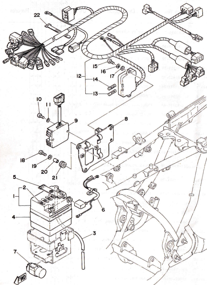
Fig. 42 ELECTRICAL 1
