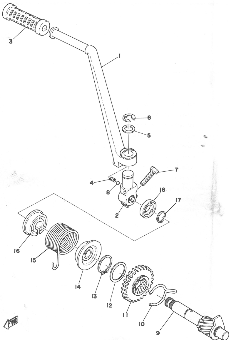
Fig. 8 KICK STARTER
