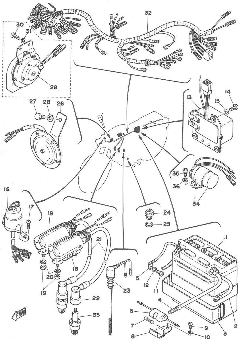
Fig. 40 ELECTRICAL
