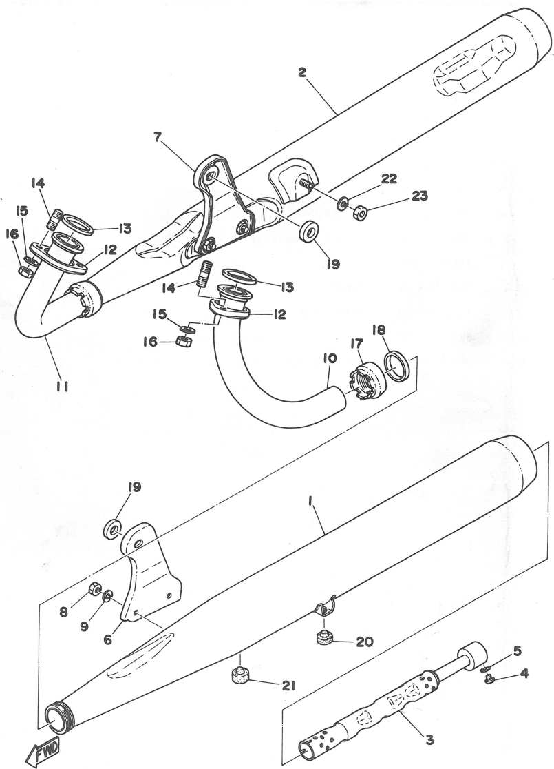
Fig. 12 EXHAUST
