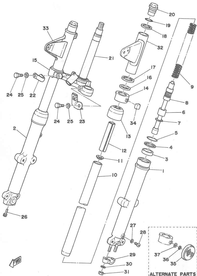
Fig. 21 FRONT FORK
