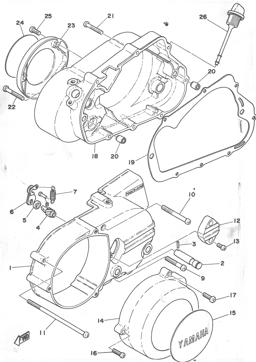
Fig. 2 CRANKCASE COVER
