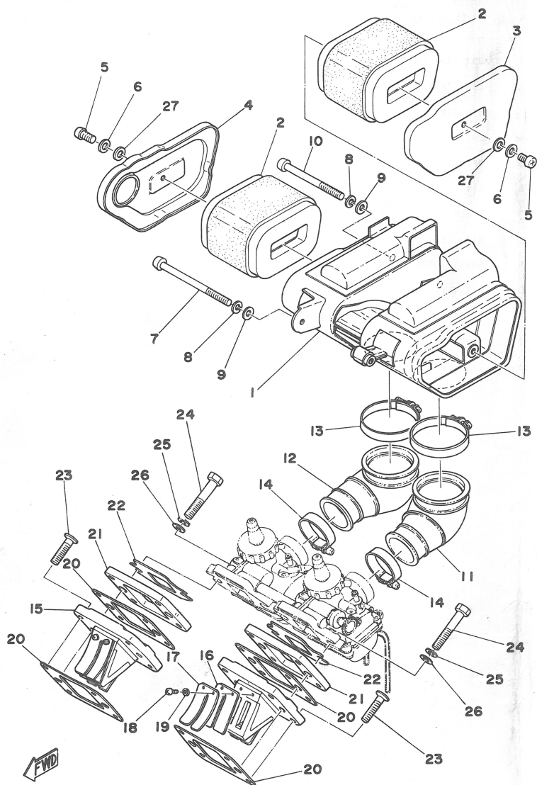
Fig. 10 INTAKE
